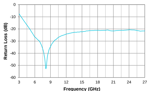
Return Loss
